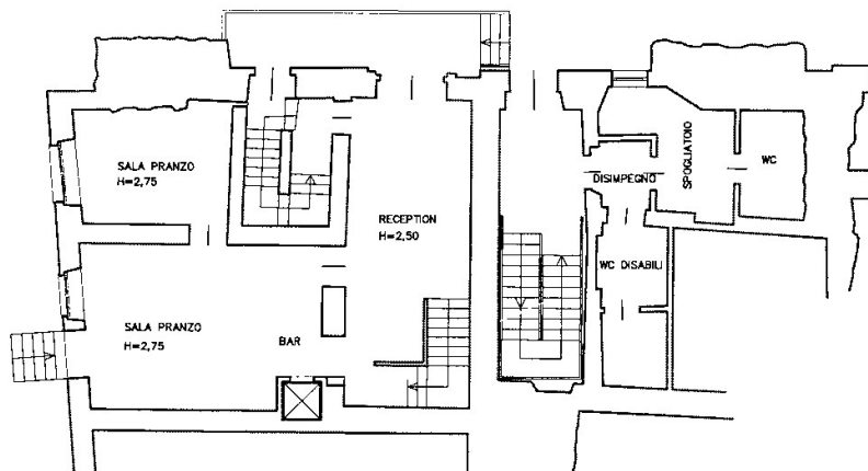
PIANO TERRENO
