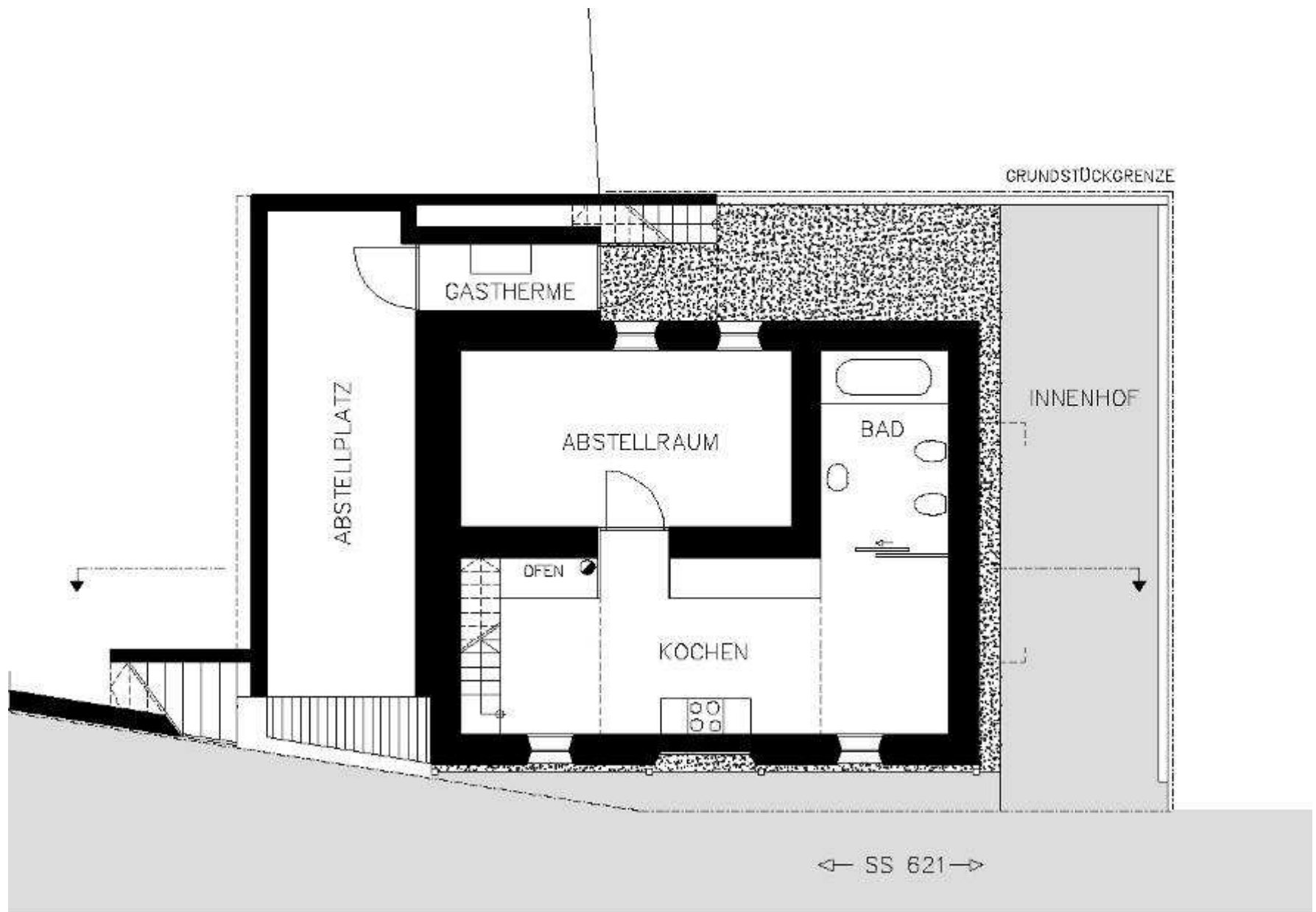
PIANO SEMINTERRATO
